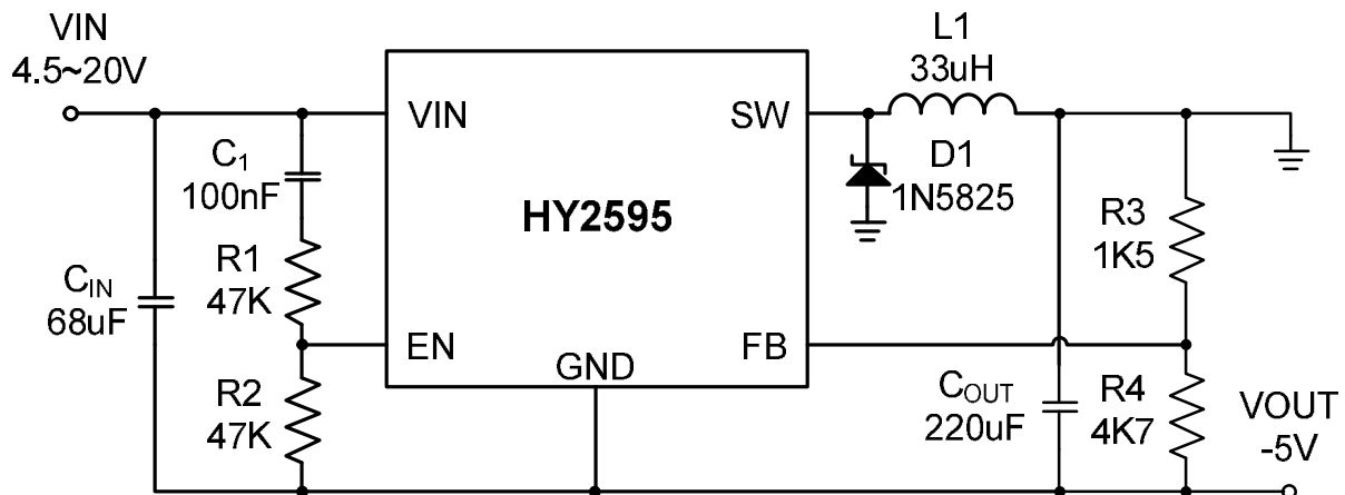
Inverting -5V Regulator with Delayed Startup
