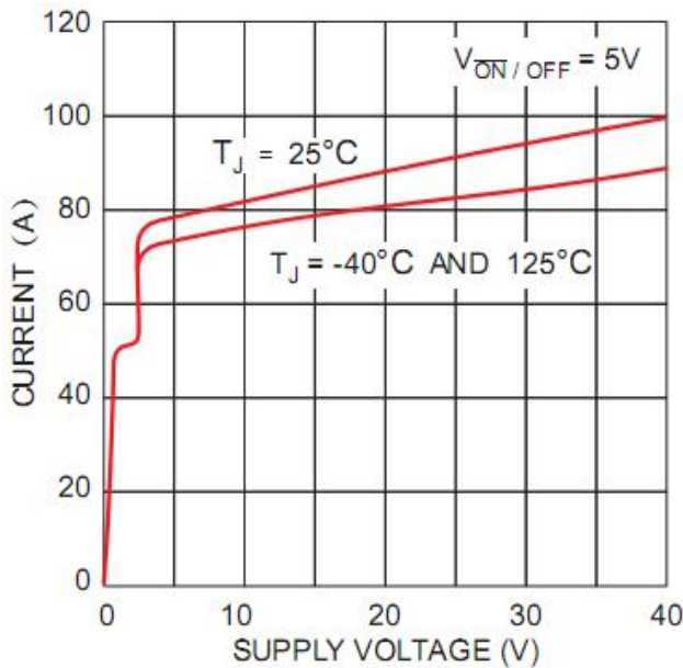
Shutdown Quiescent Current
